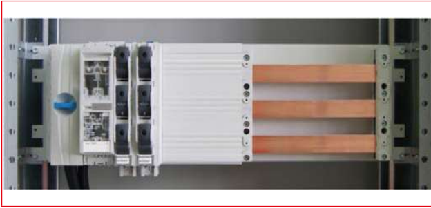
Mounting Example 60 mm System
